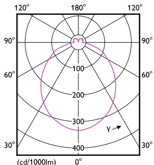
Light Distribution Diagram - Corepro LEDspot 550lm GU10 840 120D
